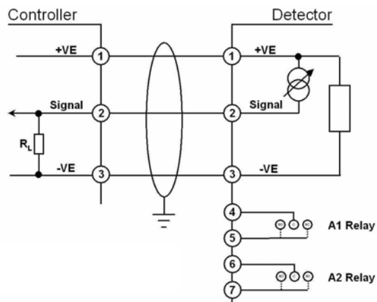
3 Wire 4-20mA (Source) + Relays
